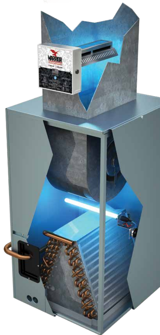
Air handler installation with optional 2nd remote UV light
